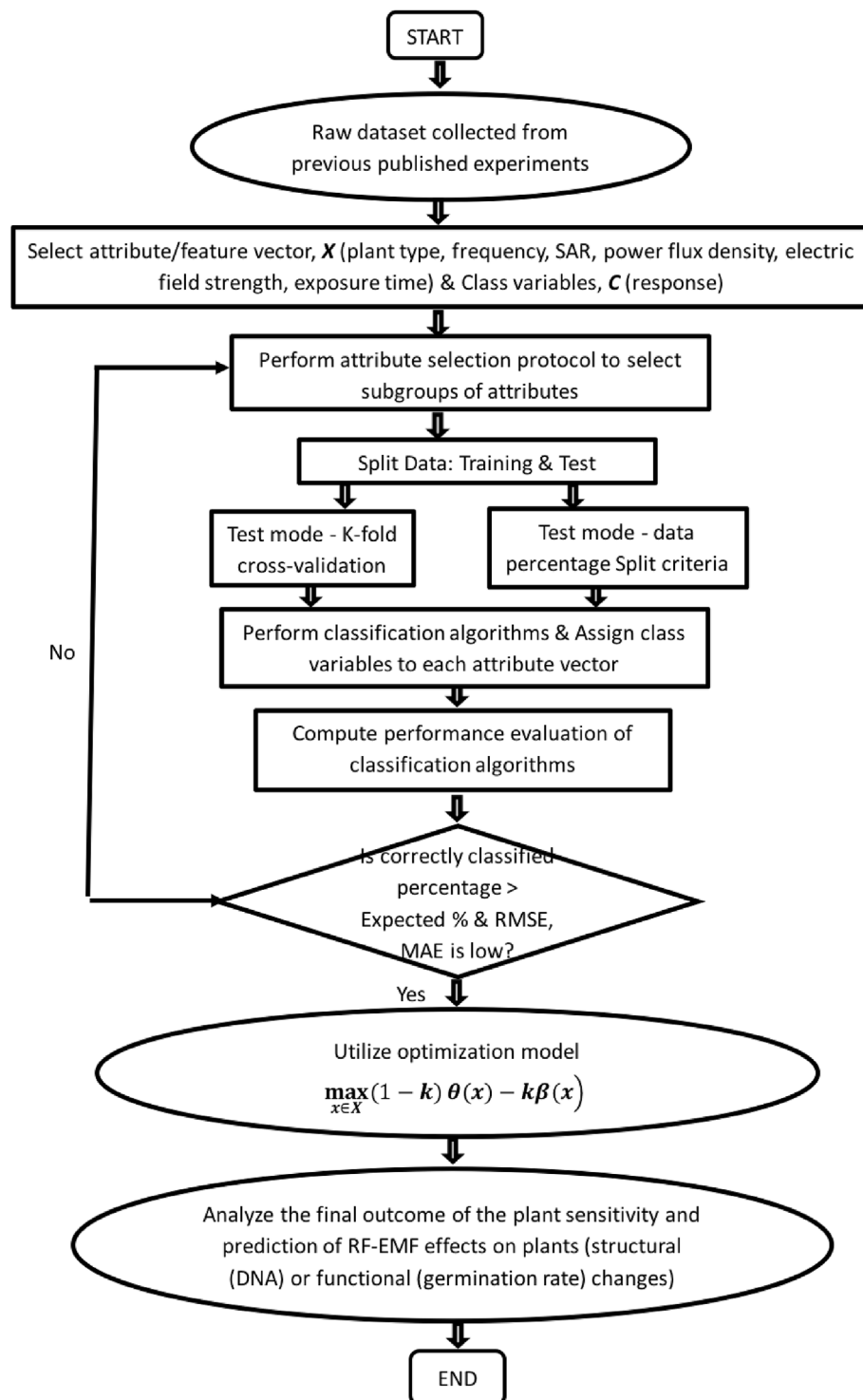
Fig. 2. Flow chart to predict plant sensitivity to radio-frequency electromagnetic field (RF-EMF).
