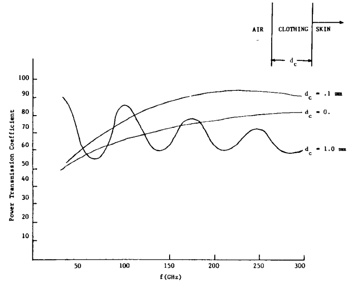
Fig. 4. Comparison of transmission coefficient with and without clothing ( d_a = 0 ).
