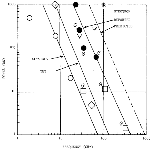
Fig. 1. Microwave tube power: ( \square ) published Russian CW gyrotron data; ( \bullet ) Russian millisecond pulsed gyrotrons; ( \circ ) klystrons; ( \diamond ) TWT's and extended interaction klystrons; ( \blacklozenge ) millisecond pulsed gyrotron; ( \nabla ) CW gyrotron; ( * ) Russian 100- \mu s pulsed gyrotron (from [5]).
