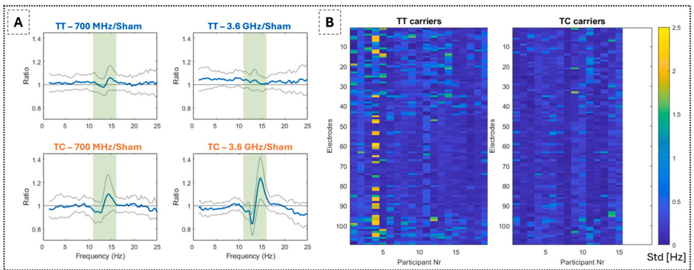
Fig. 3. A) Mean ratio (blue lines) of whole-night, sleep EEG power density spectra (1–25 Hz, 0.25-Hz bins) between exposure conditions (700 MHz and 3.6 GHz) and sham in T/T ( n = 19 ) and T/C ( n = 15 ) allele carriers of CACNA1C in EEG derivation C3 referenced to the right mastoid (C3-RM). Green shading indicates the spindle frequency range (11–16 Hz). Grey lines indicate the 95 % CI. B) Intra-subject standard deviation of the selected spindle peak frequency in all 109 analyzed EEG electrodes of the three nights for each participant in the T/T and T/C group. The participant number is on the x-axis and the electrode number on the y-axis. Color-coding indicates the standard deviation of the selected peaks in Hz.
