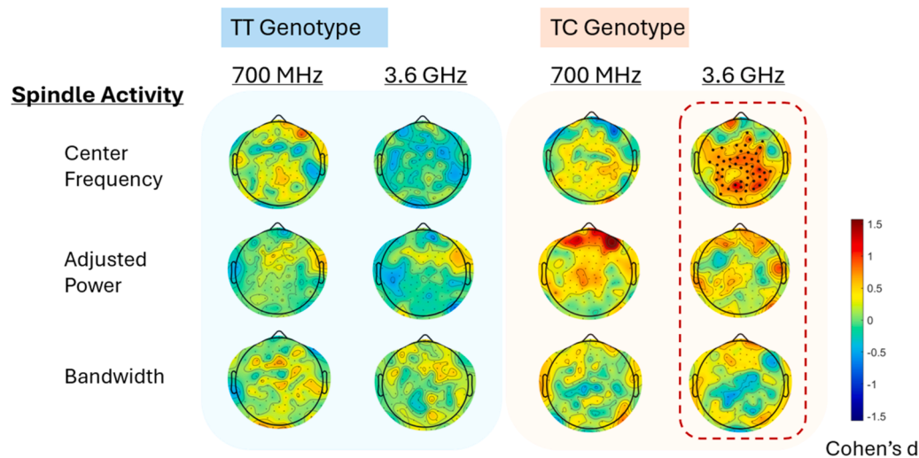
Fig. 4. Topographical distribution of the effects of the two active fields (700 MHz and 3.6 GHz compared to sham) for both allelic variants (T/T: n = 18 and T/C: n = 15 ) for the extracted variables center frequency, adjusted power, and bandwidth in the first NREM sleep episode (combined stages N2 & N3). Cluster-based permutation statistics were applied, and significant cluster electrodes ( p < 0.05 ) are indicated by black dots. The color bar indicates Cohen's d effect sizes of the statistical comparison with sham exposure. Warm colors indicate an increase, and cold colors indicate a decrease compared to sham exposure.
