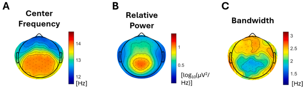
Fig. 2. Sleep Spindle Peak Parameterization. Topographical characterization of FOOF spindle peak detection ( n = 33 ; sham condition). (A) center frequency of the detected spindle peaks (Hz). (B) spindle peak power relative to the 1/f background activity ( \log_{10}(\mu V^2/Hz) ). (C) bandwidth of detected spindle peaks (Hz). Different color-codes refer to each panel.
